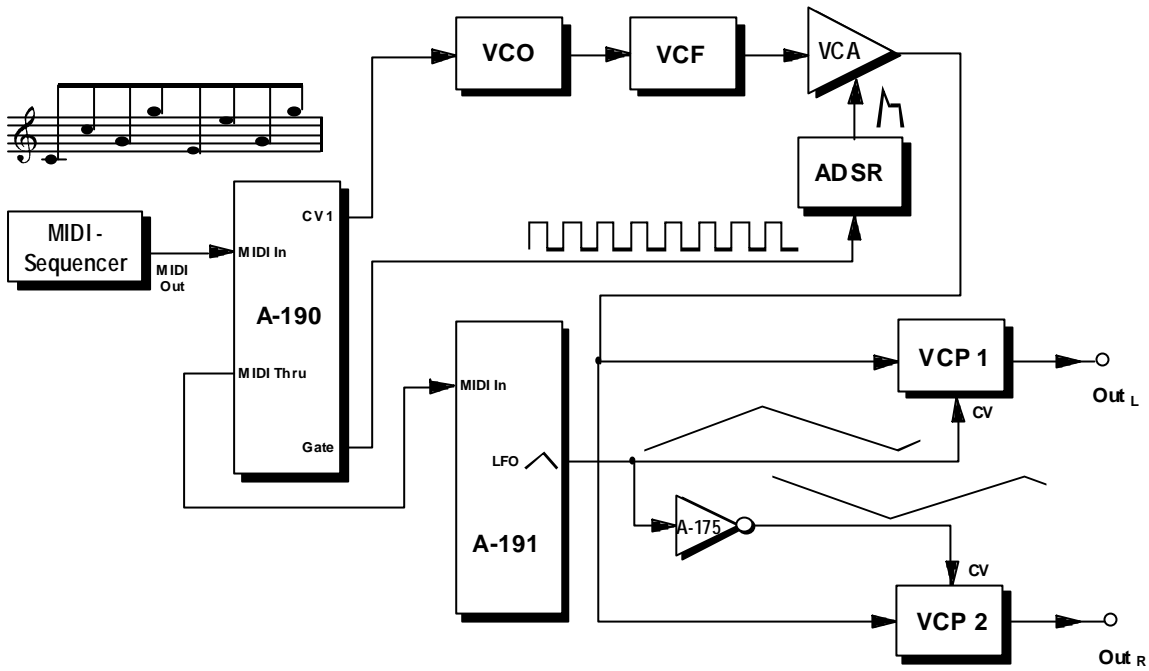
Fig. 4: MIDI-synchronised "stereo" phasing.
