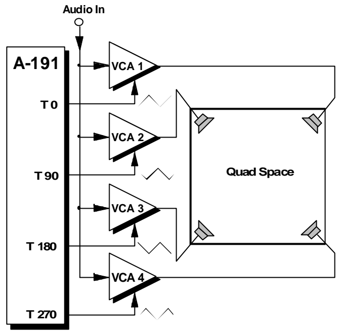
Fig. 9: Patch for quadraphonic spatial effects
