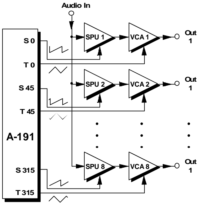
Fig. 8: Patch for Shepard control of signal processing
